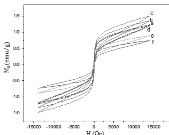
Fig. 8. Magnetization diagram (VSM) of 20SiO 2 -50FeO-30CaO glass-ceramic samples heat treated at a) 520°C, b) 600°C, c) 680°C, d) 440°C, e) 760°C and f) 840°C.
