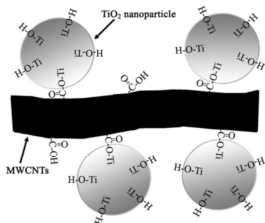
Fig. 6. Schematic illustrating the possible chemical interaction between the m modified MWCNTs and \text{TiO}_2 nanoparticles.
