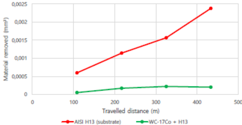
Fig. 14. Microadhesive wear tests WC-17Co/AISI H13.
