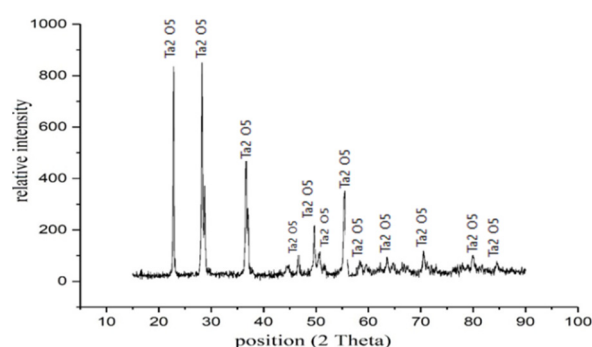
Fig. 3. X-ray diffraction patterns of \text{Ta}_2\text{O}_5 .
