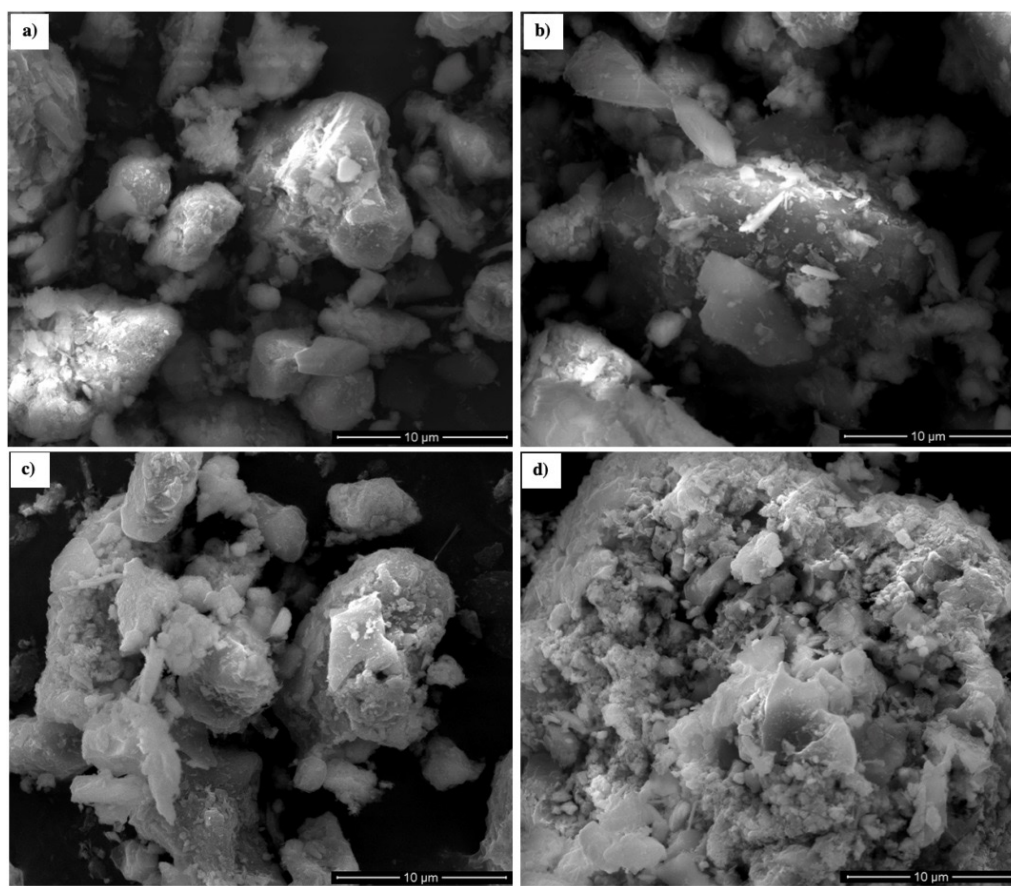
Fig.7. SEM images obtained from powders in two different particle sizes, (a) small particle size initial iron ore(180-250 \mu m) (b) big particle size initial iron ore(250-750 \mu m ) (c) small particle size iron ore roasted at 600 ^{\circ} C and 25min (d) big particle size iron ore roasted at 625 ^{\circ} C and 25min.
